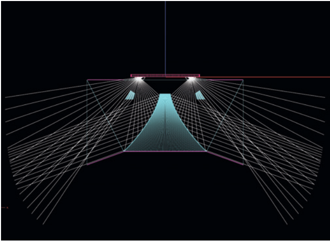
KTY200 series - Ray tracing
